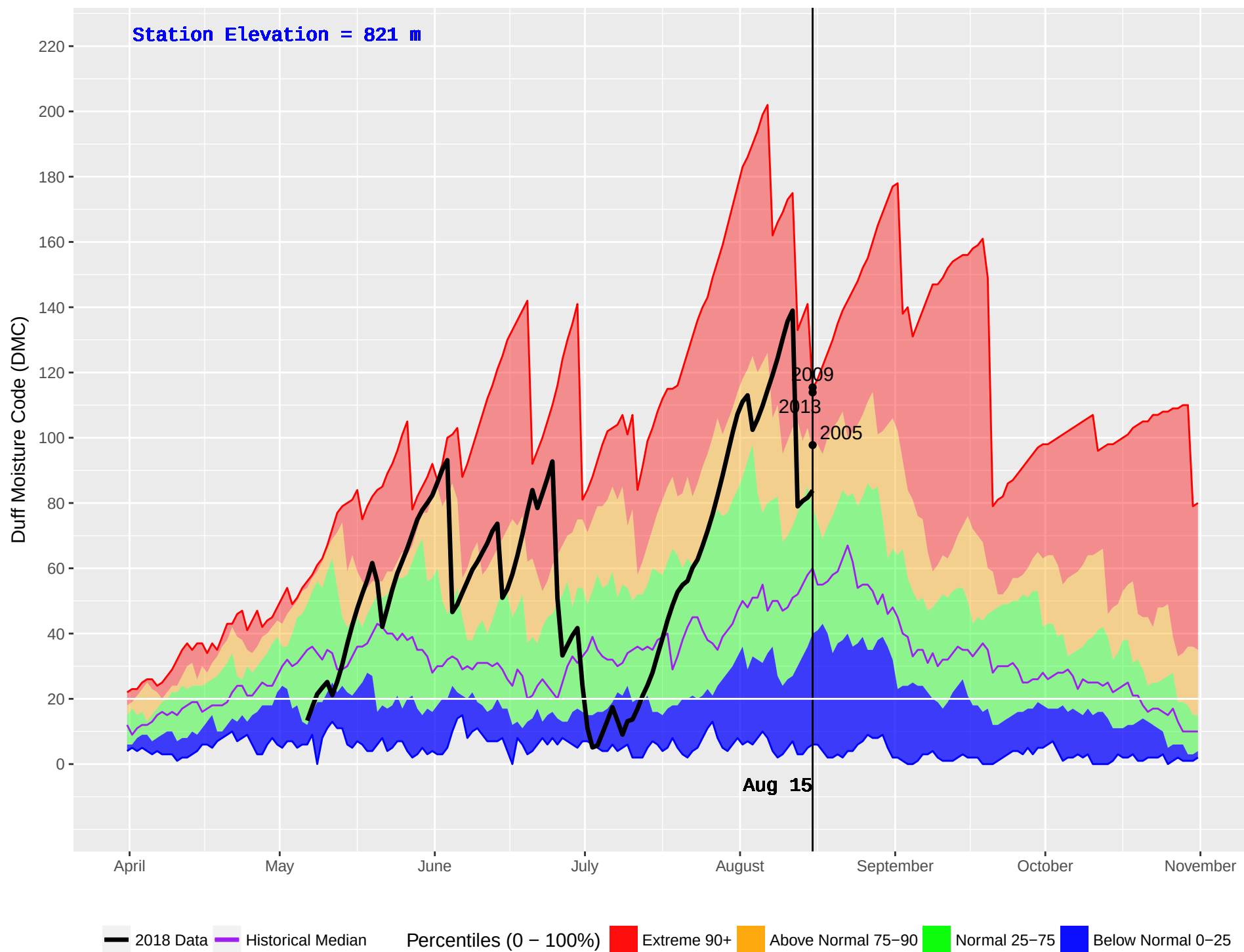
KNIFE (225) : Historical (1991–2016) and Current (2018) Daily Duff Moisture Code (DMC)
