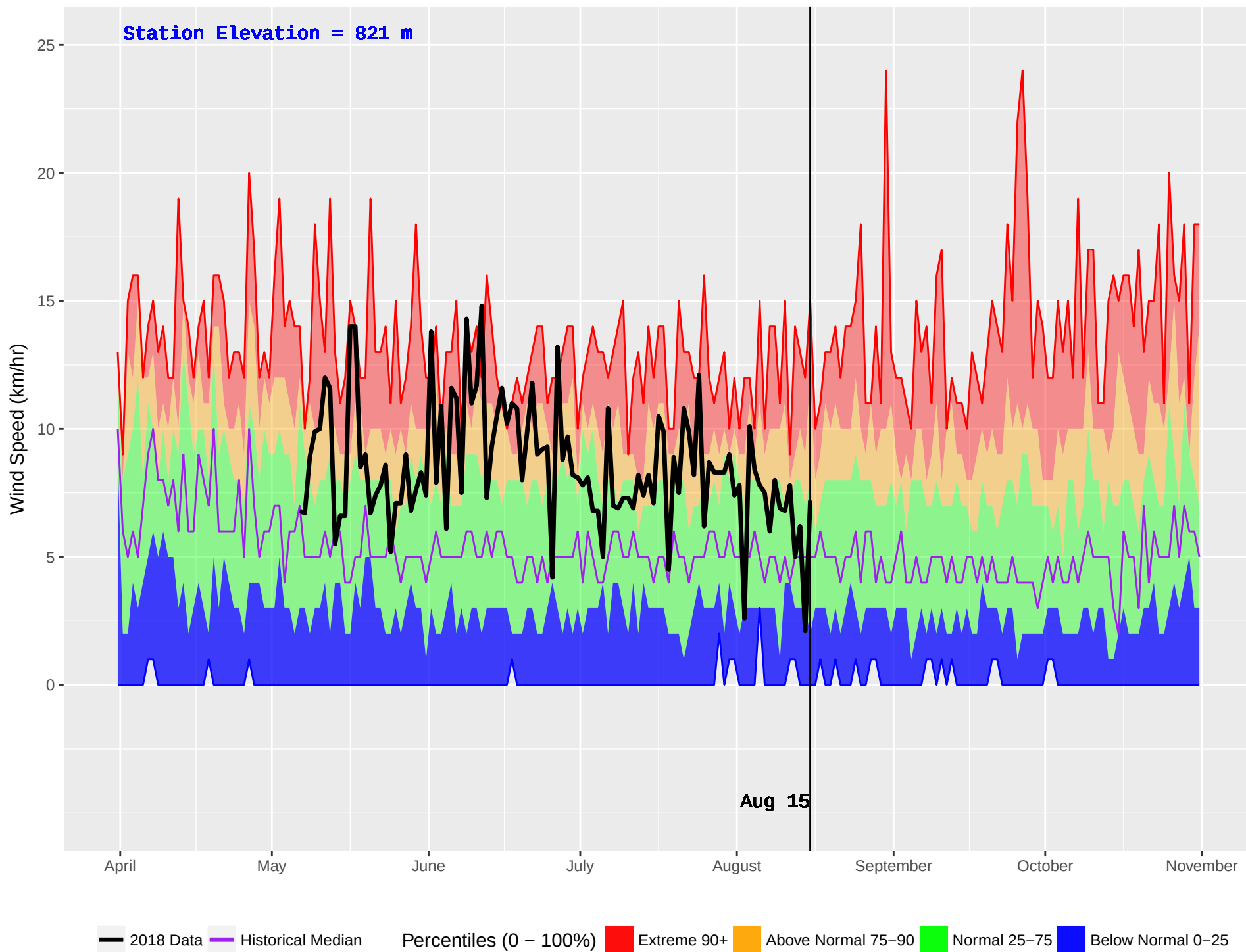
KNIFE (225) : Historical (1991–2016) and Current (2018) Daily Wind Speed
