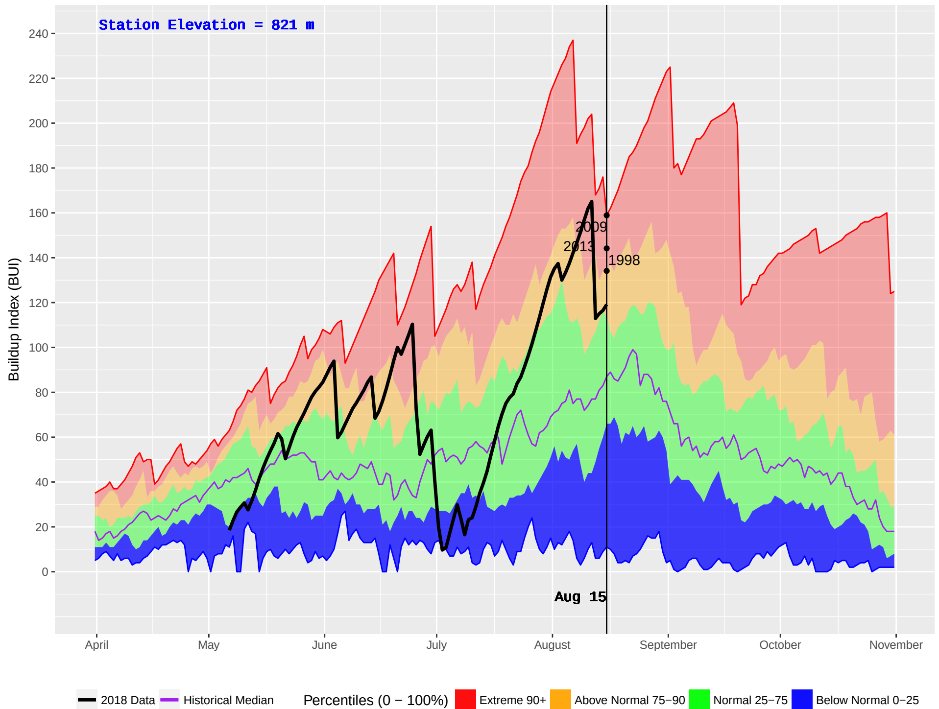
KNIFE (225) : Historical (1991–2016) and Current (2018) Daily Buildup Index (BUI)
